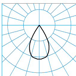
E-Line Fi B.VEO RFS-VFL 05 50-840 J17 L37 03 (150) TX124764 ■ C0 - C180
