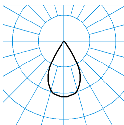
E-Line Fi B.VEO RFS-VFL 05 50-840 J17 L37 03 (225) TX124243 ■ C0 - C180
