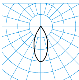
E-Line Fi B.VEO RFS-WFL 05 50-840 J17 L37 03 (225) TX123897 ■ C0 - C180
